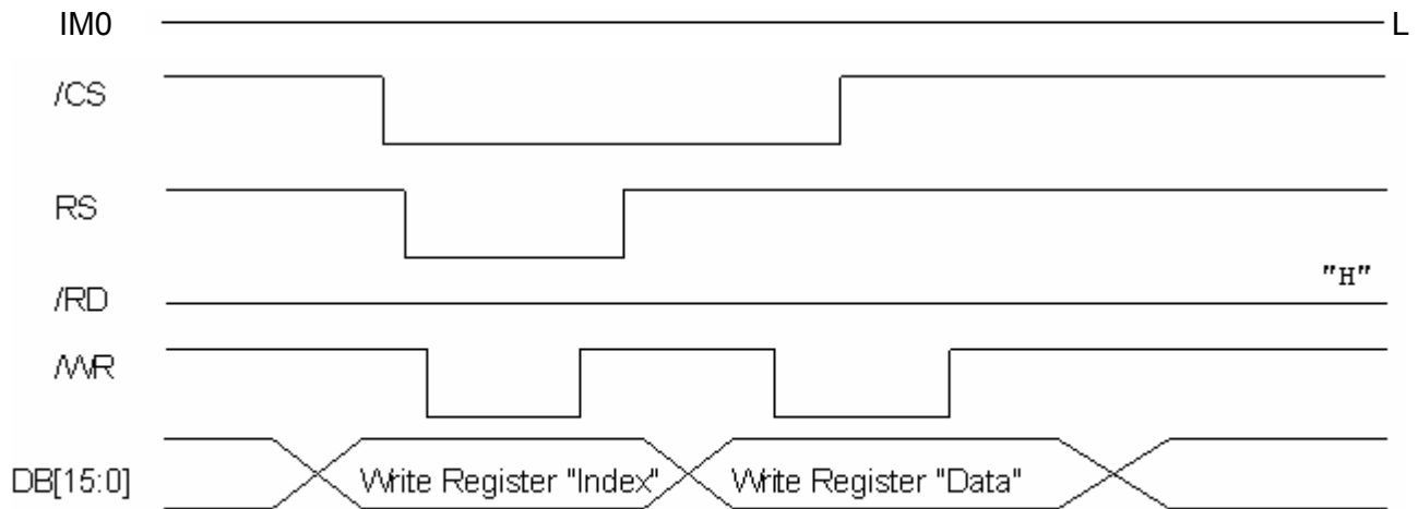
Figure 5.2.1 16-bit System Bus Interface Timing(Register Write Timing)
